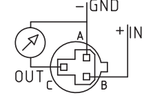
B (IN) C (OUT) A (GND)
