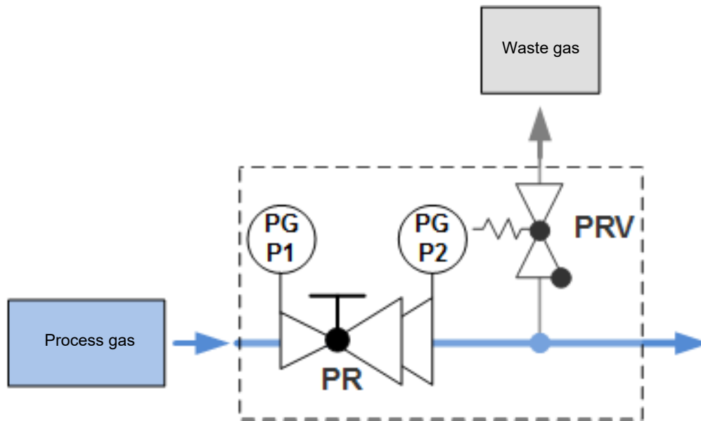
Illustration 2: P&ID E53
